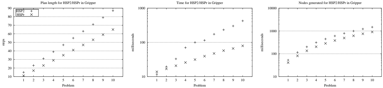
Figure 9: Comparison between HSP2/HSPPr in Gripper. Curves show solution length (left), solution (center), and number of nodes generated (right)
