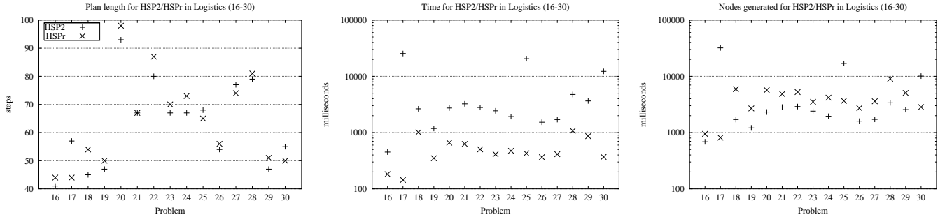
Figure 8: Comparison between HSPr vs HSP2 over Logistics instances 16–30. Curves show solution length (left), time (center), and number of nodes generated (right).
